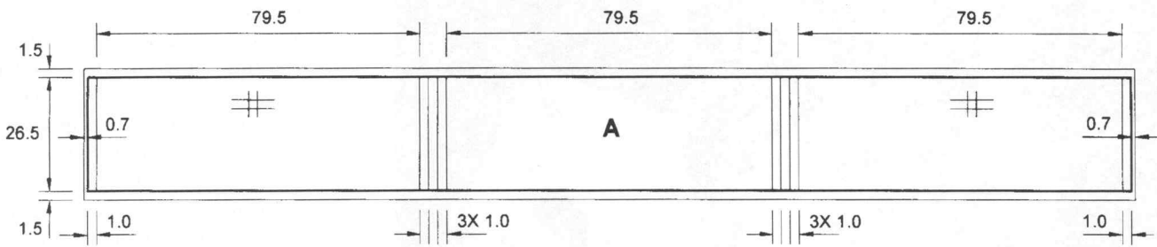
BINNENCCELLEN 2X PANEEL A
